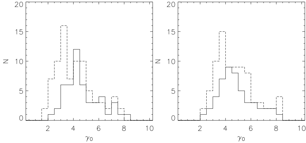
Fig. 5. Distributions of \gamma_0 for ‘centre’ ( \mu > 0.9 , dashed line) and ‘limb’ ( \mu < 0.1 , solid line) flares. The left plot corresponds to observed \gamma_0 , the right plot is for spectra corrected for isotropic albedo, i.e. with directivity \alpha = 1 .
